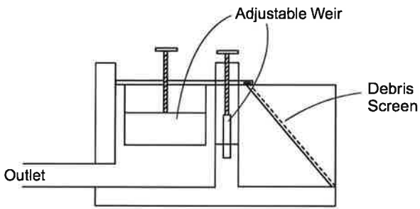
a) Adjustable Weir
