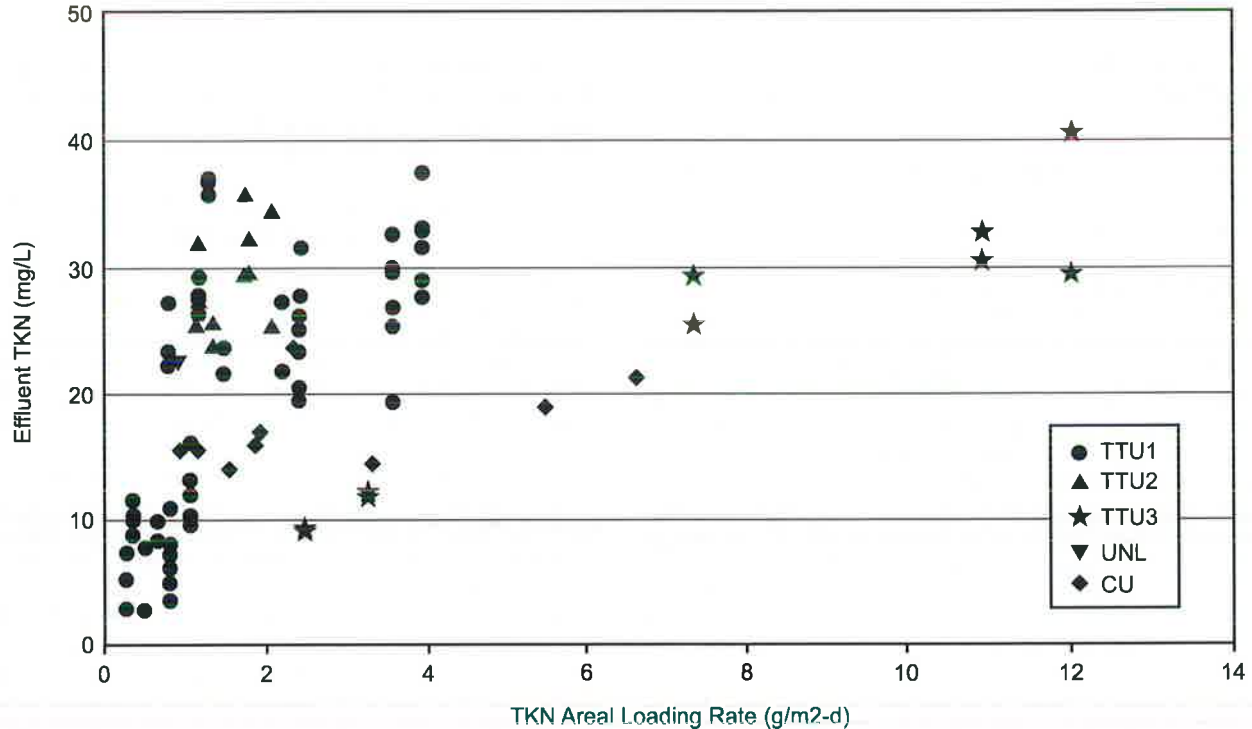
Figure 5-8. Effluent TKN vs areal loading rate
