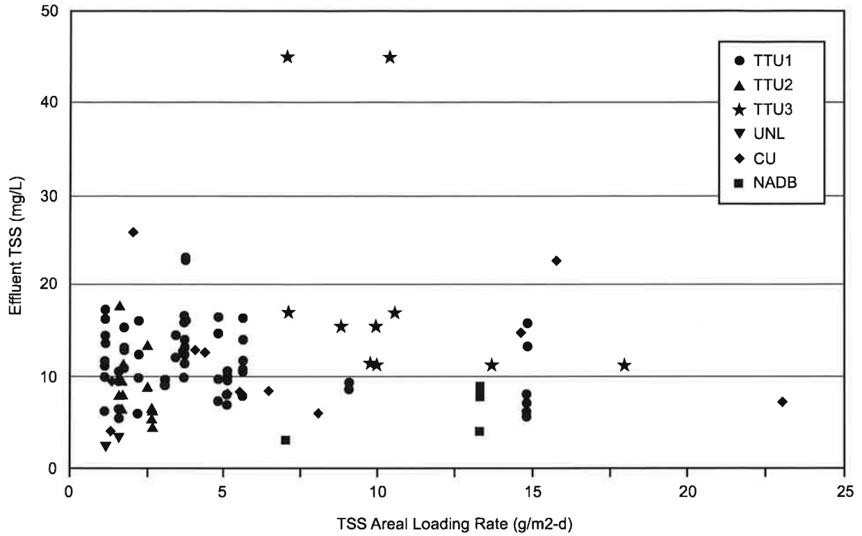
Figure 5-4. Effluent TSS vs areal loading rate
