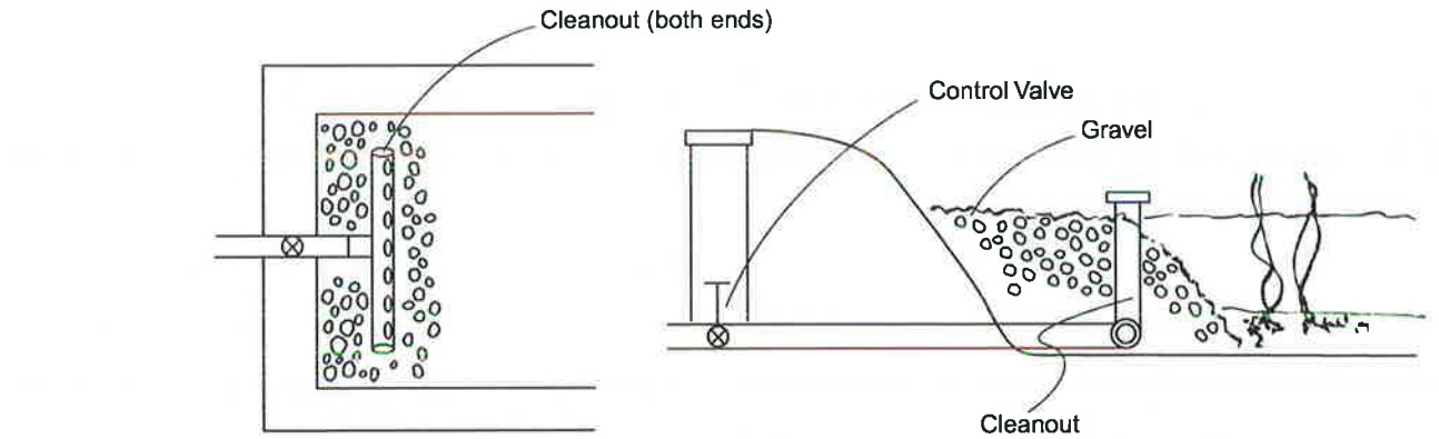
a) Submerged Perforated Pipe
