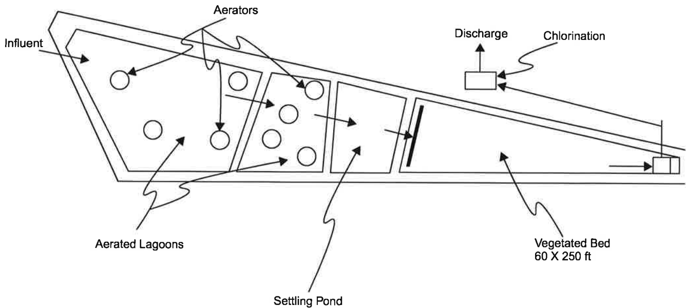
Figure 8-9. Schematic of VSB system at Sorrento, LA
