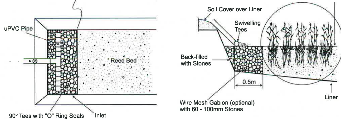
c) Swivel Tee
