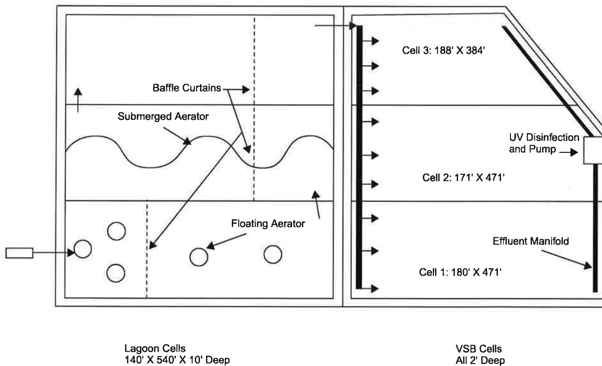
Figure 8-8. Schematic of VSB system at Mandeville, LA
