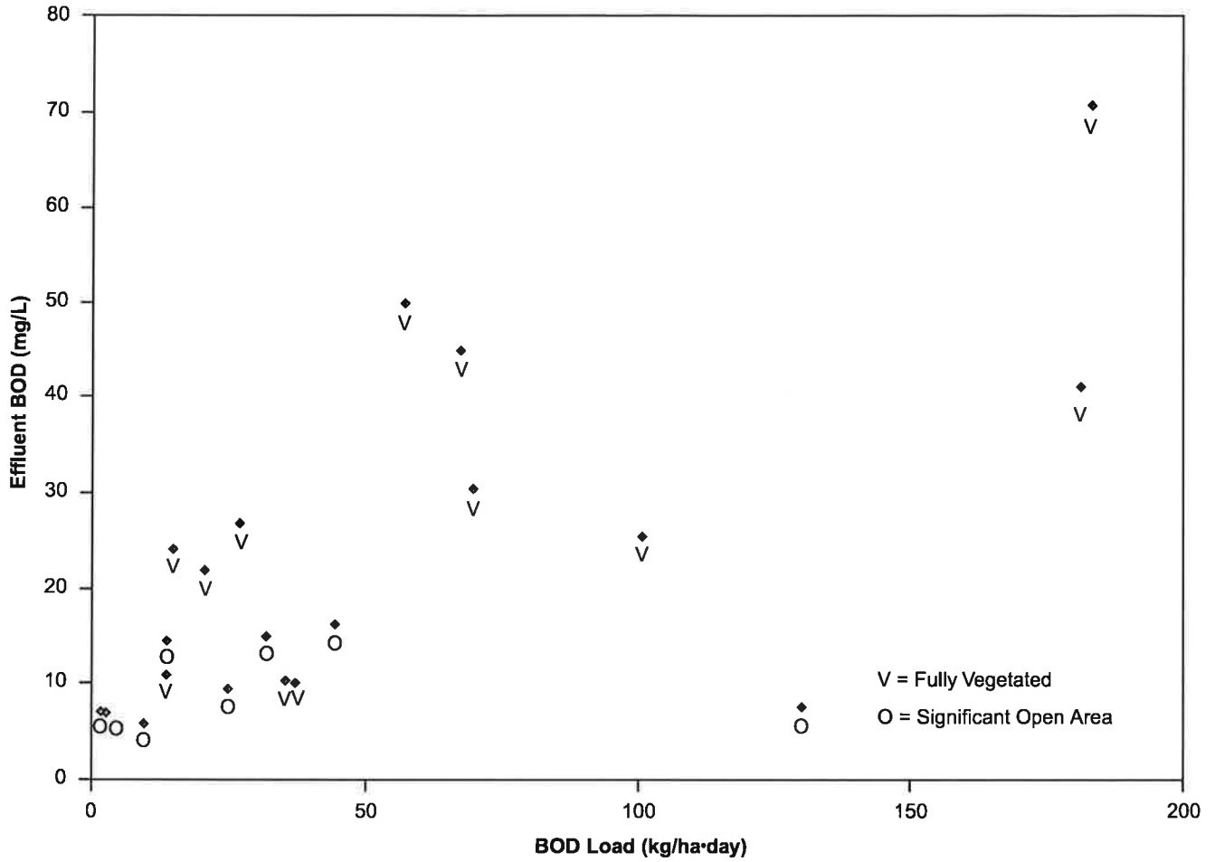
Figure 4-1. BOD effluent vs. areal loading (DMDB)
