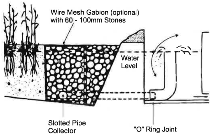
c) 90° Elbow Arrangement
