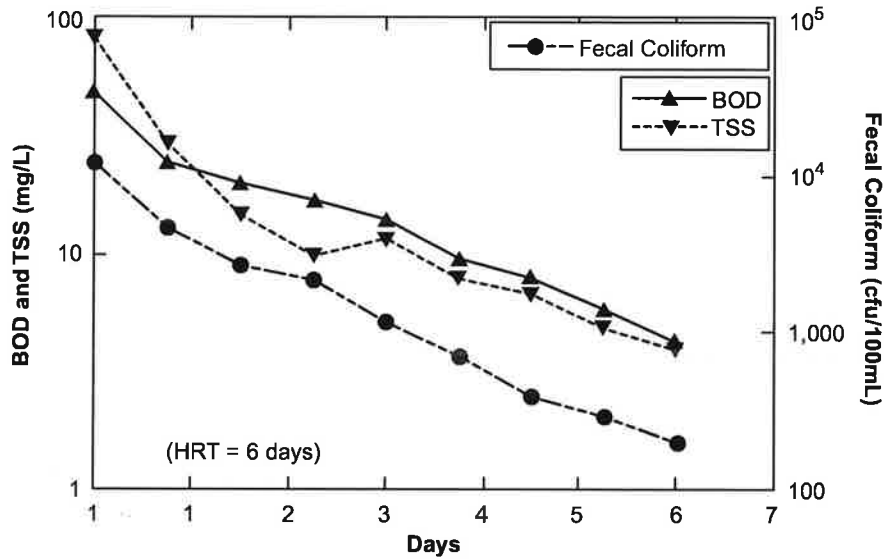
Figure 4-10. Arcata pilot Cell 8, TSS, BOD, FC
