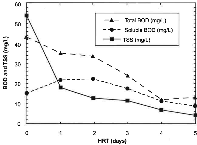
Figure 4-2. Release of soluble BOD during early stage
