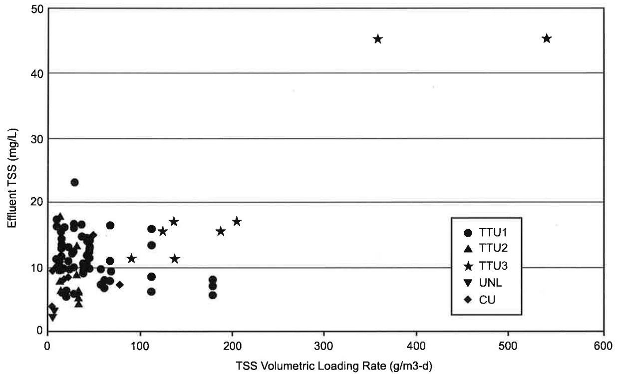
Figure 5-5. Effluent TSS vs volumetric loading rate
