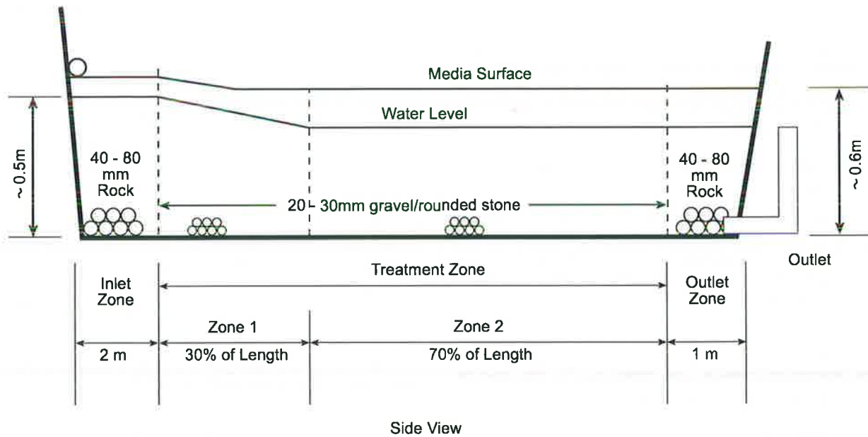
Figure 5-11. Proposed Zones in a VSB
