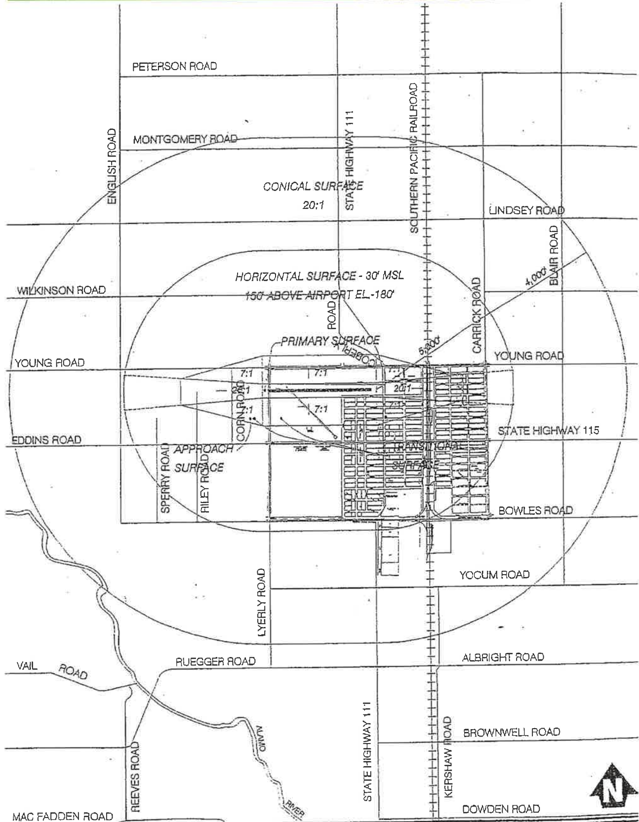
Figure A14: CALIPATRIA AIRPORT (CLR) 1996 PART 77 SURFACES
