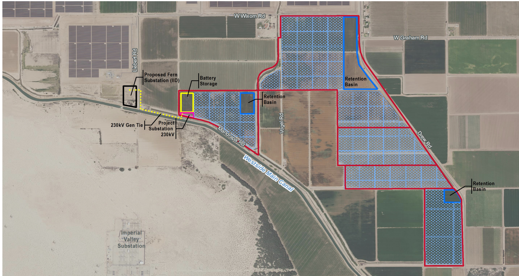
Figure 2. Previously-Approved VEGA SES Solar Energy Project – Site Plan
