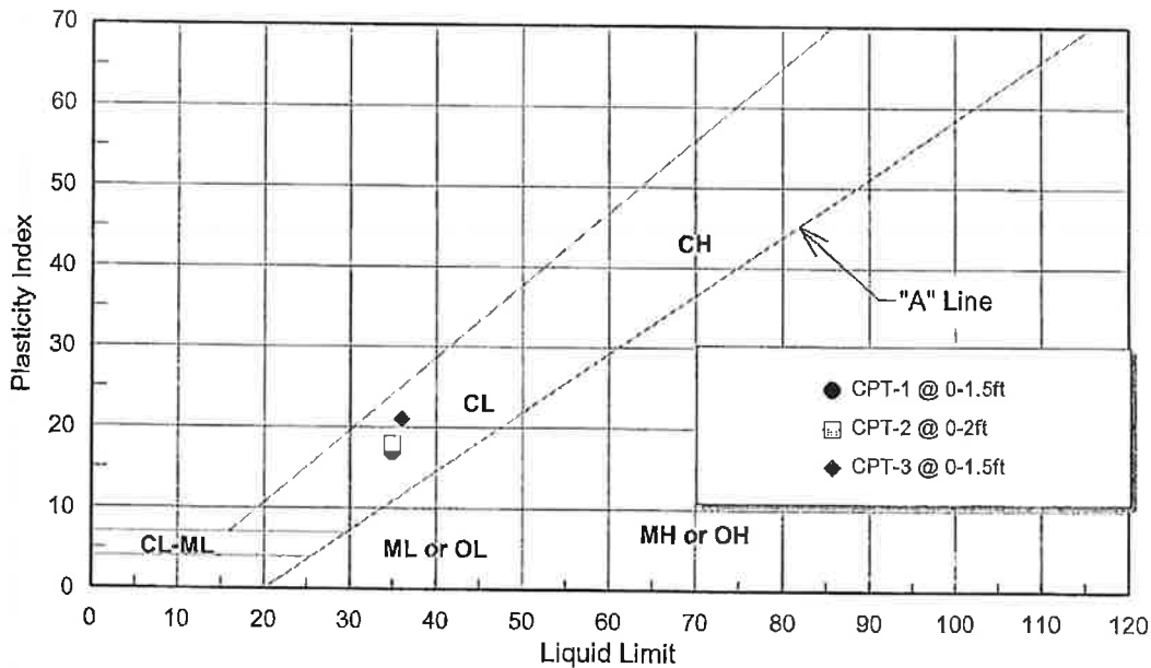
PLASTICITY CHART
