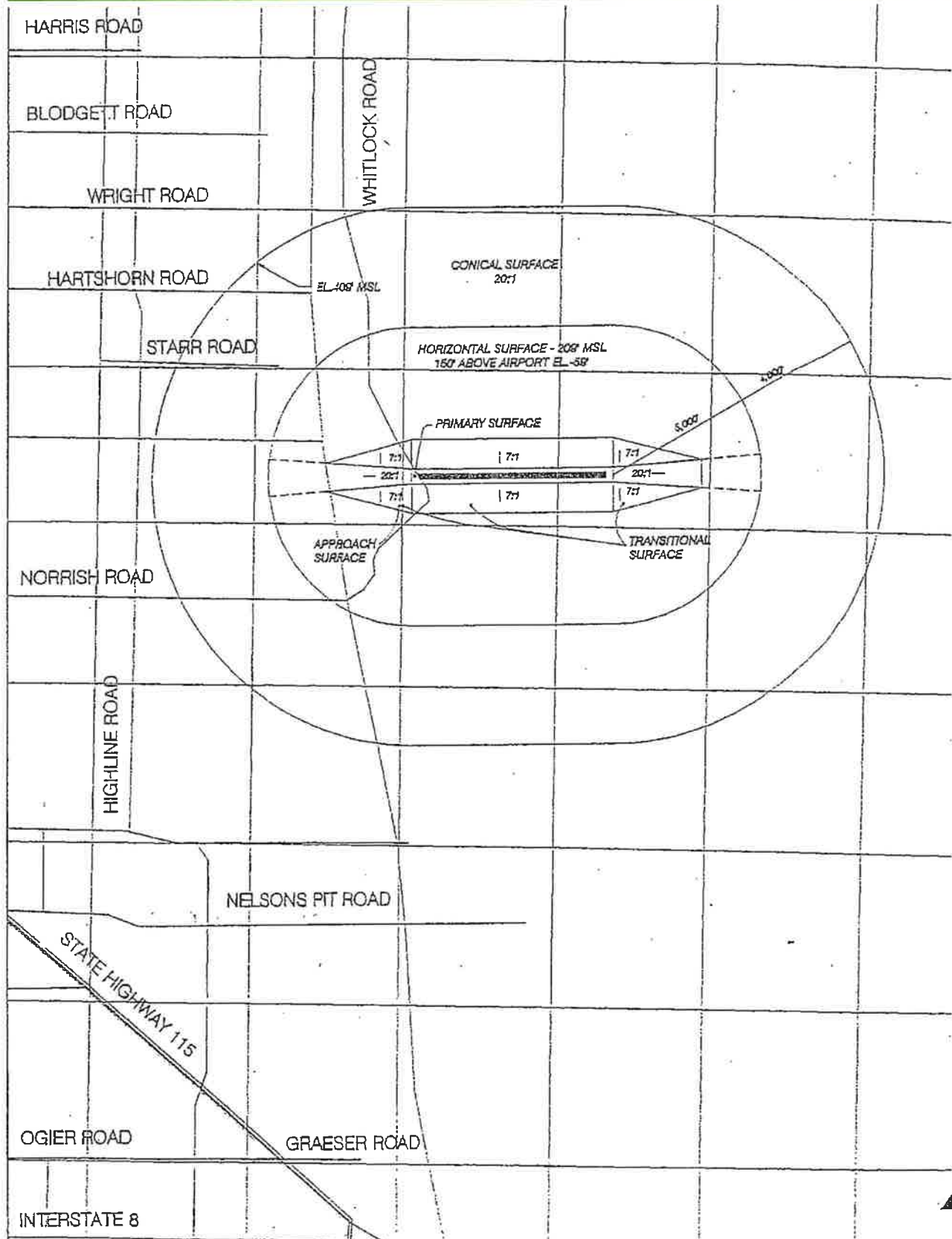
Figure A15: HOLTVILLE AIRPORT (L04) 1996 PART 77 SURFACES
