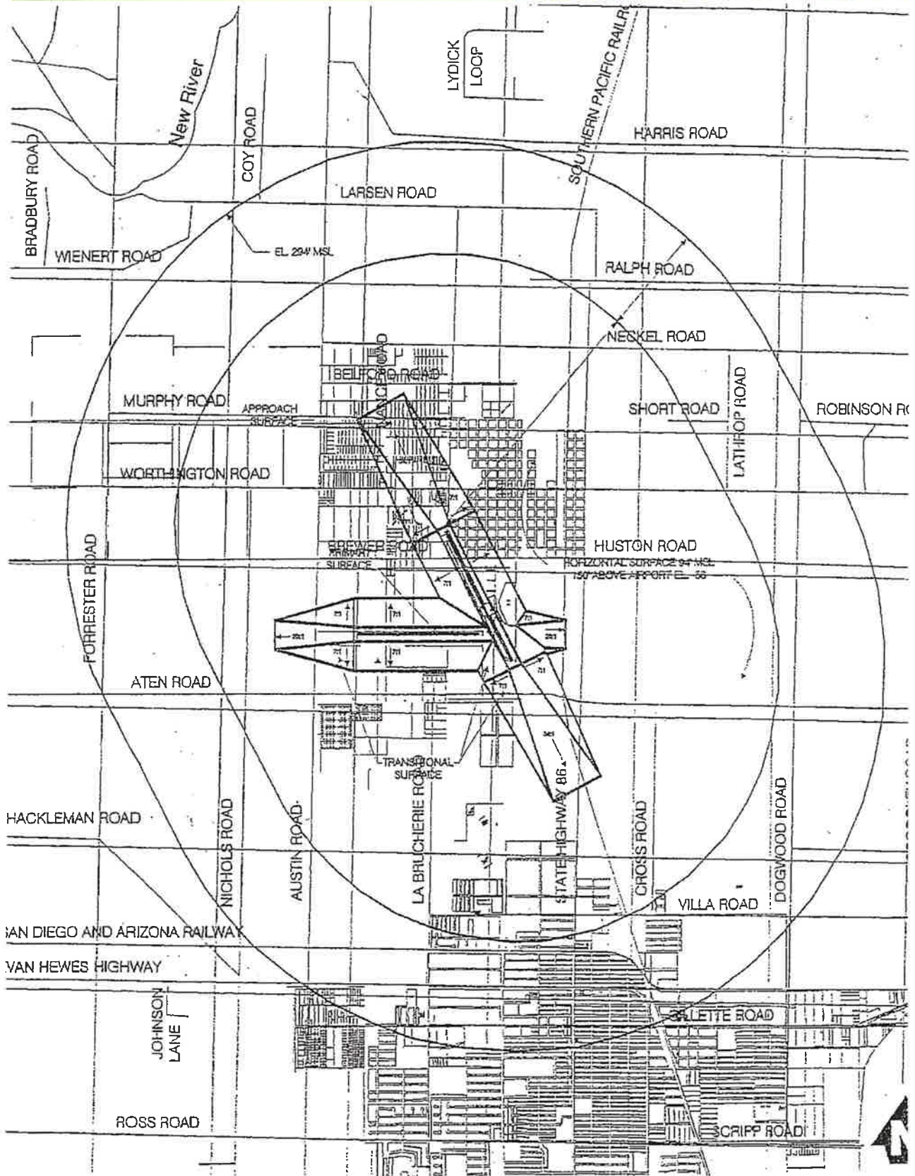
Figure A16: IMPERIAL COUNTY AIRPORT (IPL) 1996 PART 77 SURFACES
