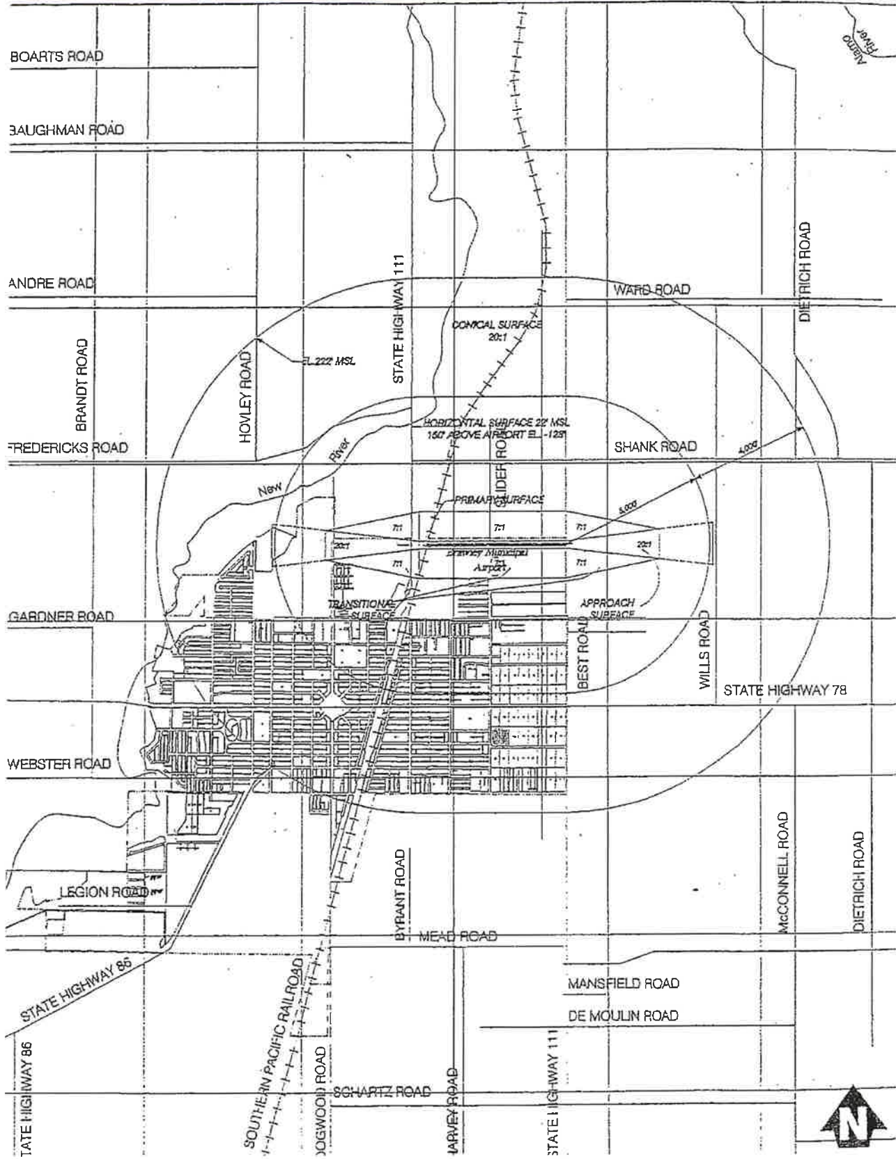
Figure A12: BRAWLEY MUNICIPAL AIRPORT (BWC) 1996 PART 77 SURFACES
